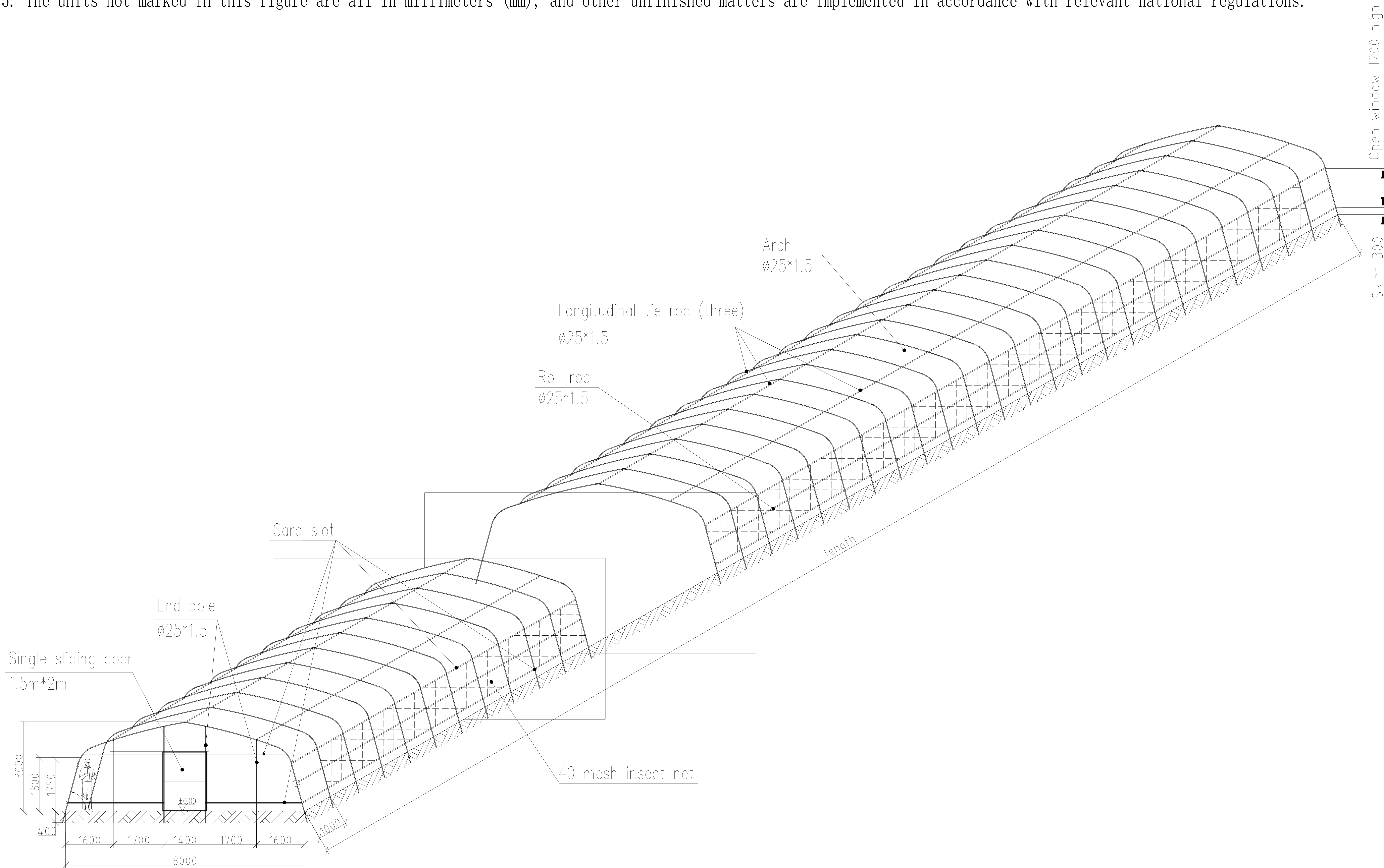
Perspective view of 8m span standard single room shed
